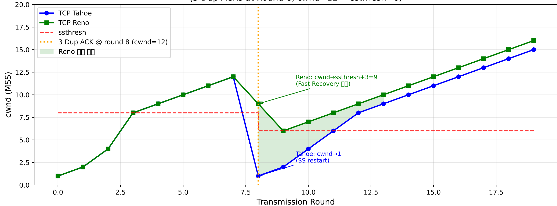
TCP Tahoe vs. Reno: cwnd Evolution (3 Dup ACKs at Round 8, cwnd=12 \rightarrow ssthresh=6)
